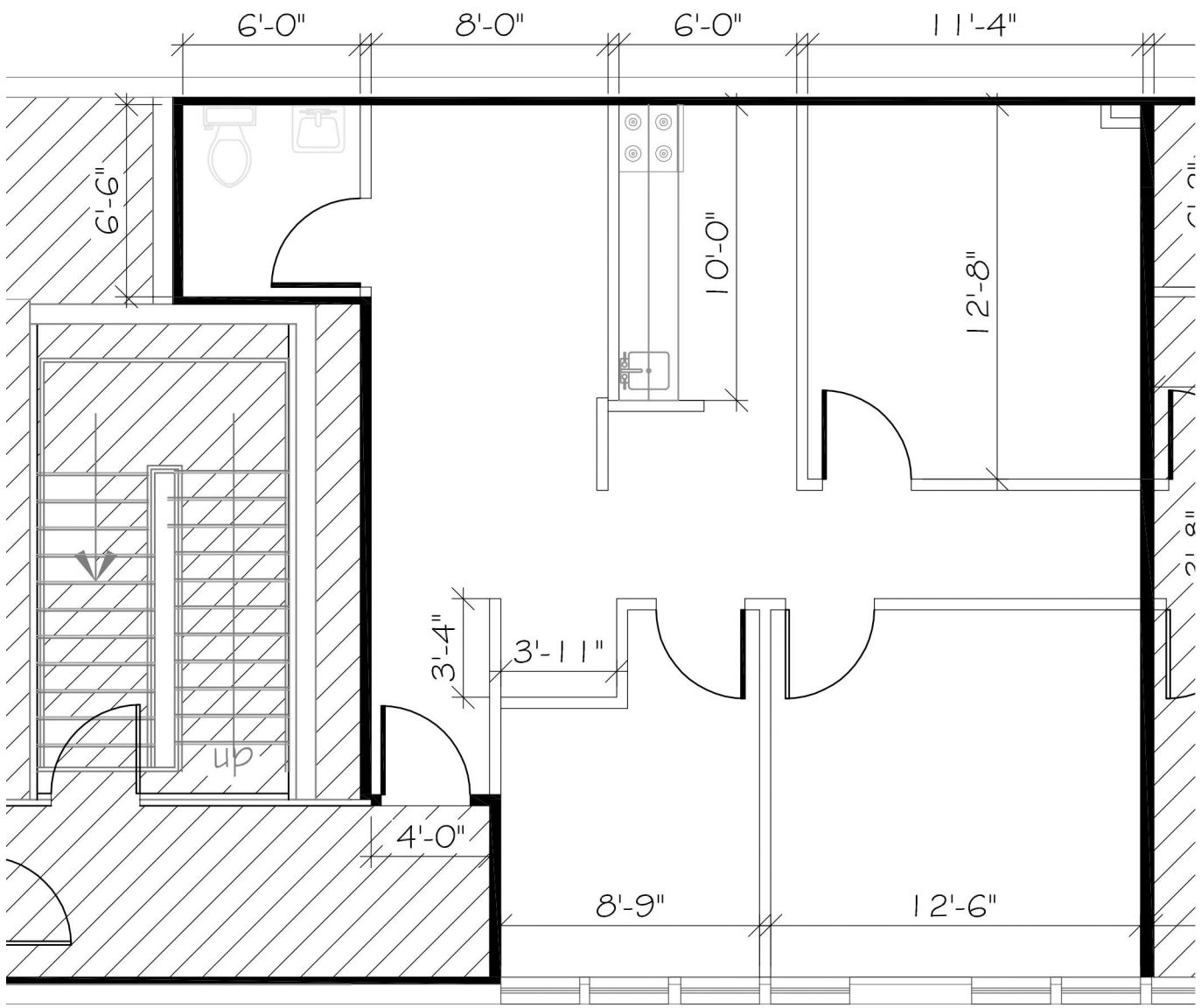
FLOOR PLAN - KITCHEN AND LIVING AREA
